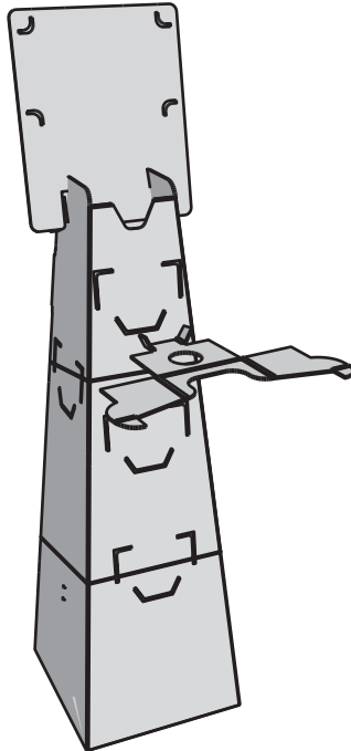
6. Insert bottom pocket tabs into slots on front of base.
